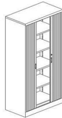
ZA-0919 W900 x D470 x H1920 ZA-1019 W1000 x D470 x H1920 ZA-1219 W1200 x D470 x H1920
